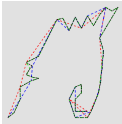
Fig. 24: Geomtransform generalize
