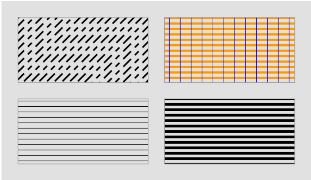
Fig. 9: Hatch examples
