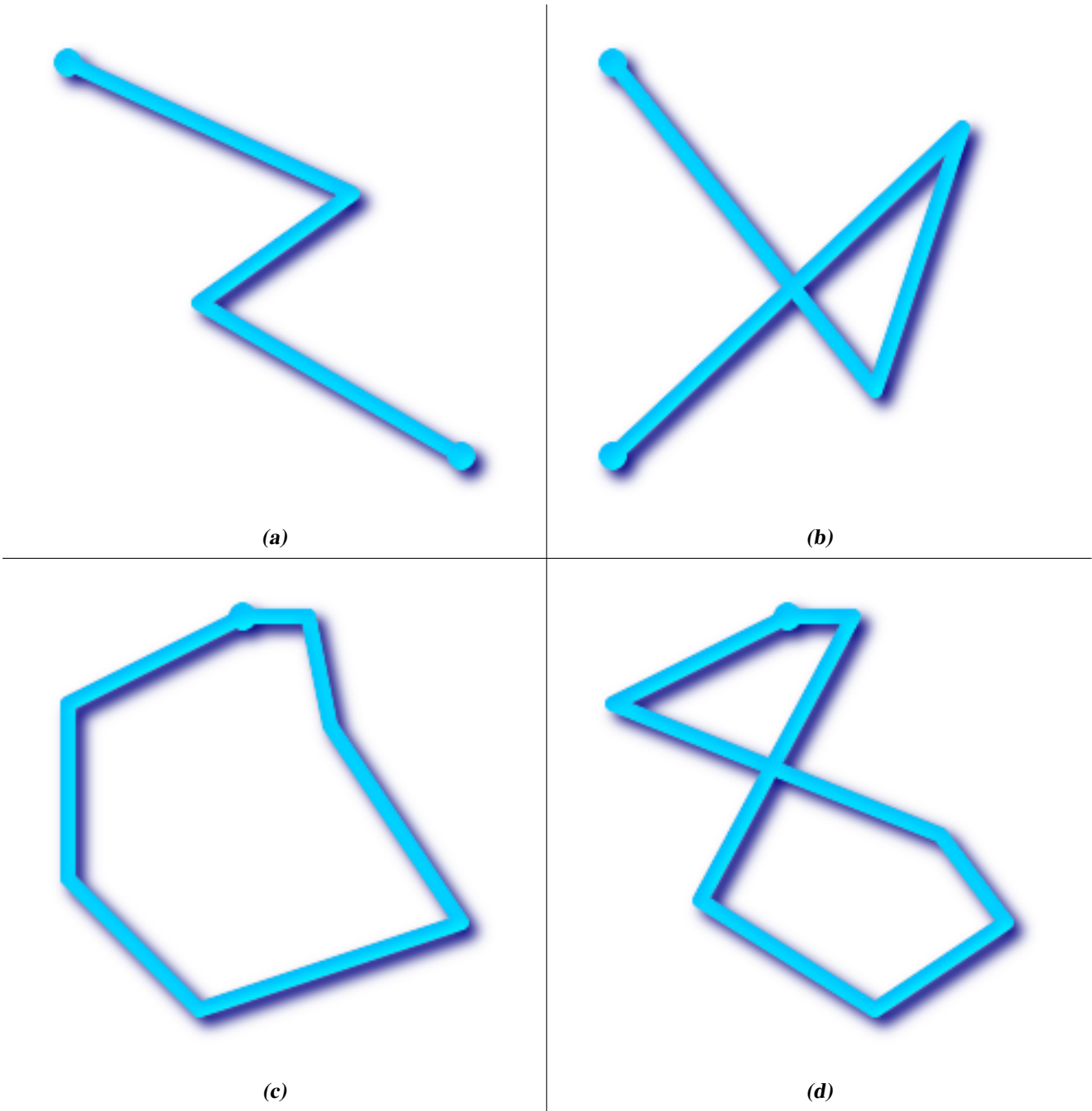
(a) and (c) are simple LINESRINGS, (b) and (d) are not.
